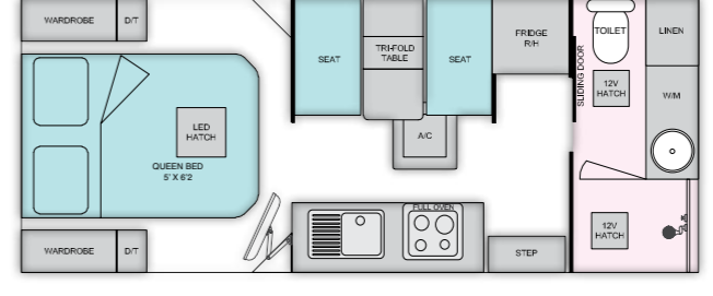
VAN 1-1 - 18'8"
