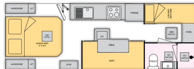
FAMILY 2-5 - 21'10"
