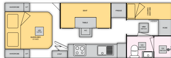
FAMILY 3 - 22'10"
