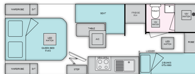
FAMILY 1-5 - 20'6
